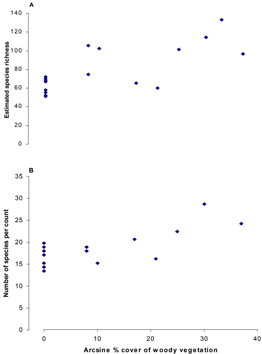
Figure 3(A). Total bird species richness (from Jack-knife estimates) increases with the amount of woody vegetation, as represented by % cover: values for the height bands 3-8 and >8 metres were summed ( r = 0.724 , P < 0.01 ). (B) Mean species numbers per one-hour TSC is less dependent upon trees ( r = 0.137 , NS).
